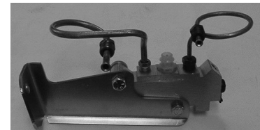
B-44 Prop. Valve, Brkt & Lines
