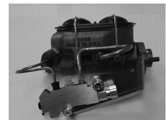
Proportioning Valve with Dual Master Cyl. Attached
