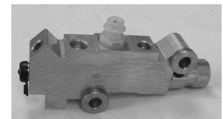
B-55 Proportioning Valve
