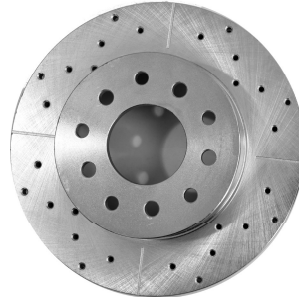
B-75-R Rear Drilled & Slotted Rotor
